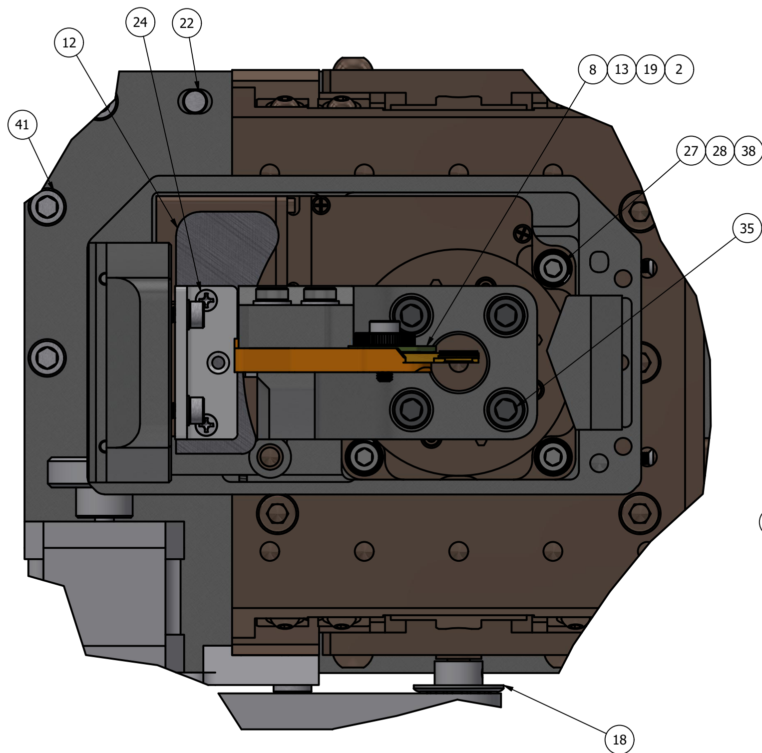
DETAIL A
